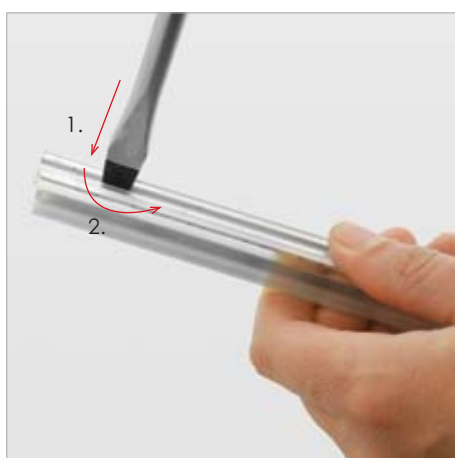
Should you not be able to slide the diffuser off due to the nature of the installation, please use a flat screwdriver as leverage applying steps 1 and 2 at different intervals along the profile
