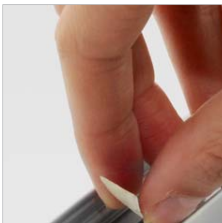
Remove the application tape from LEDtape and apply to Zero surf.
